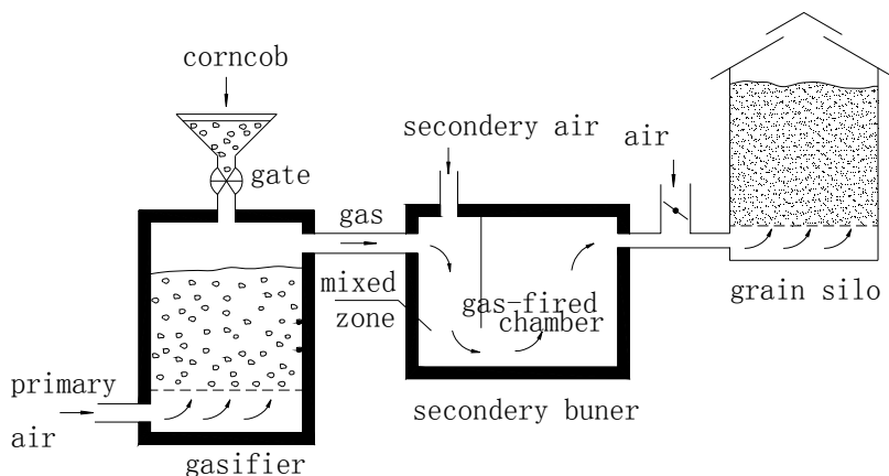
Figure3 Schematic diagram of grain drying system by means of biomass gasification
