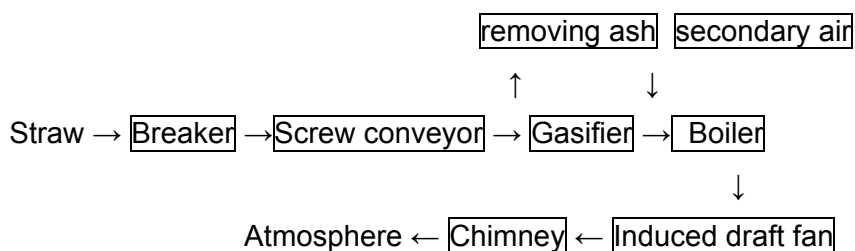
Figure 4 Principle diagram of new straw gasified-heating set
