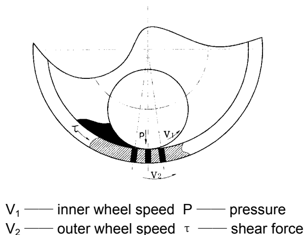
Figure 2. Schematic Diagram of Briquetting Mechanism
